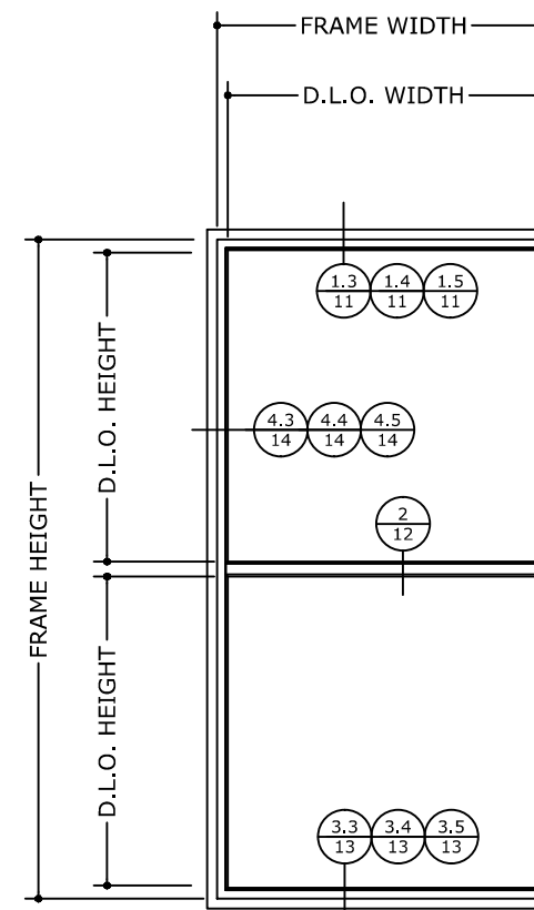
TYPICAL FIXED ELEVATION WITH INTERMEDIATE HORIZONTAL AND RECEPTOR
