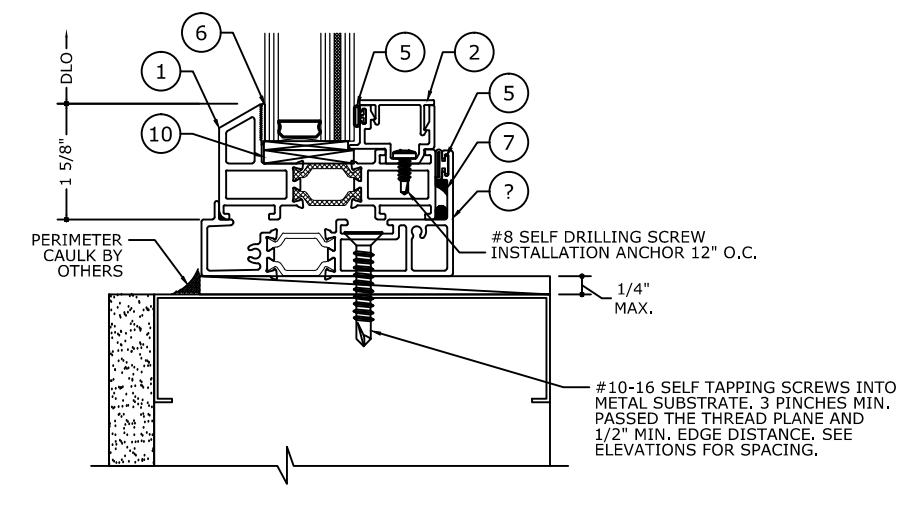
3.5 SILL DETAIL RECEPTOR
