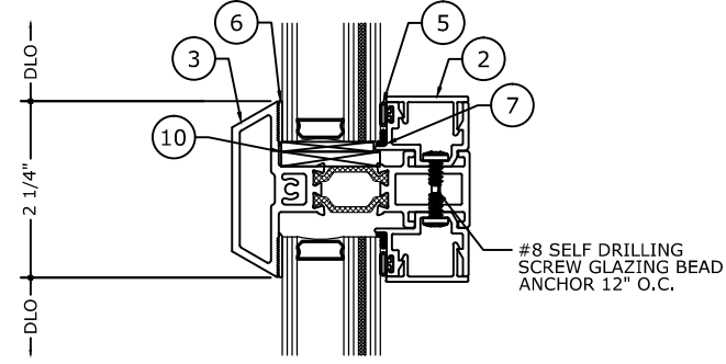
2 INTERMEDIATE DETAIL
