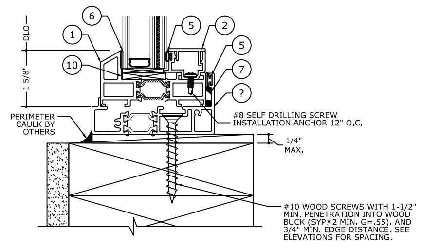
3.4 SILL DETAIL RECEPTOR
