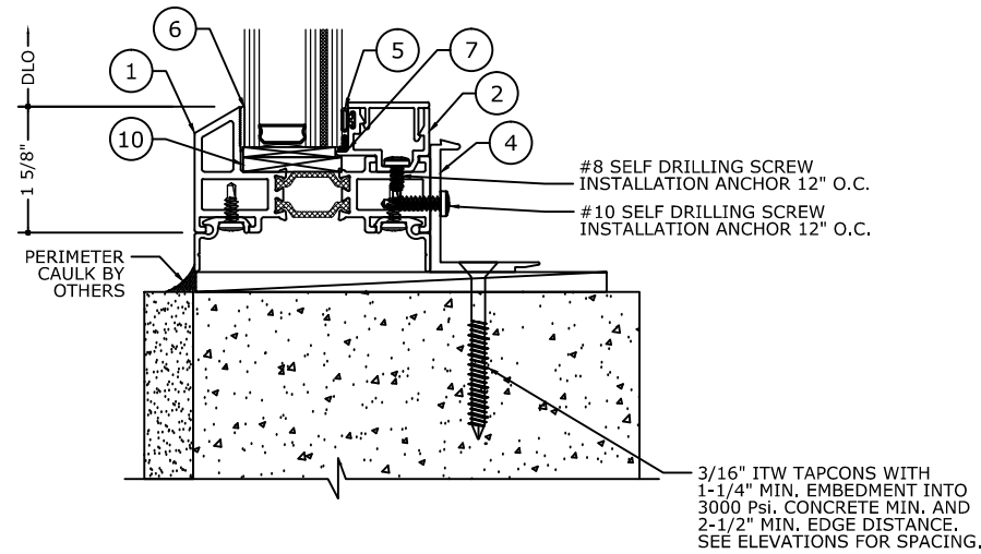
3 SILL DETAIL PRE-SET PANNING SCREW APPLIED BEAD
