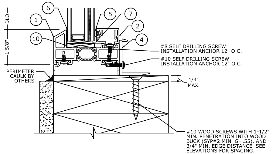
3.1 SILL DETAIL PRE-SET PANNING SCREW APPLIED BEAD
