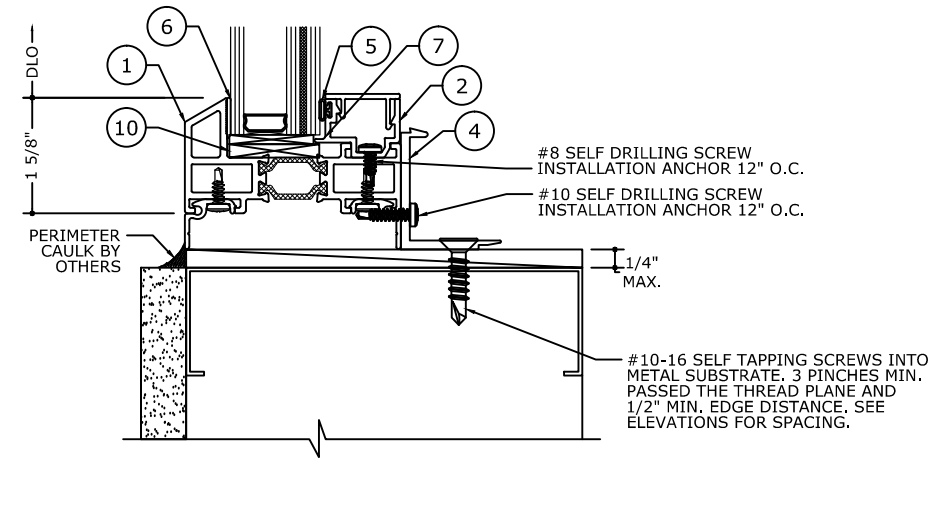
3.2 SILL DETAIL PRE-SET PANNING SCREW APPLIED BEAD
