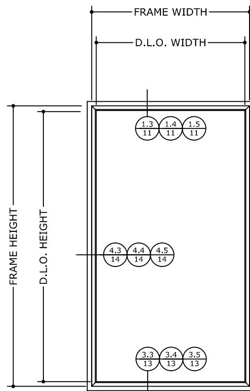
TYPICAL FIXED ELEVATION WITH RECEPTOR
