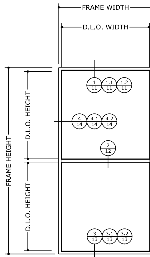
TYPICAL FIXED ELEVATION WITH INTERMEDIATE HORIZONTAL
