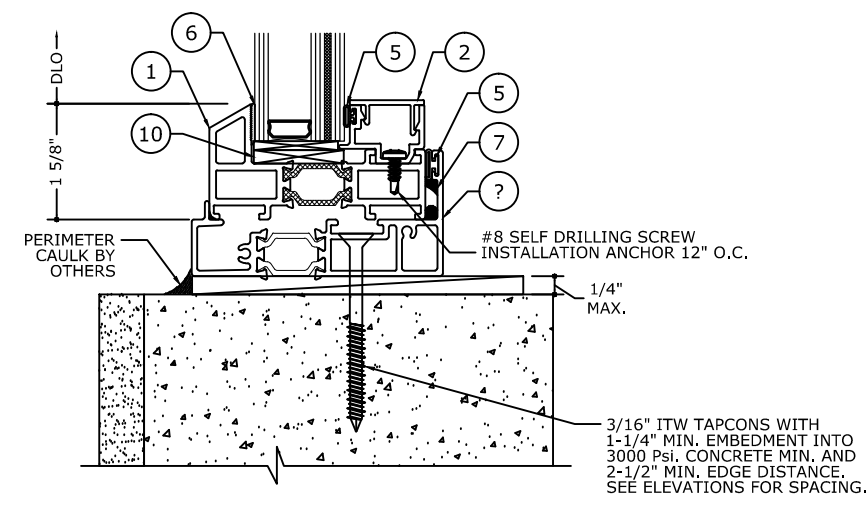
3.3 SILL DETAIL RECEPTOR
