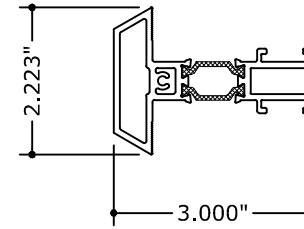
③ NARROW INTERMEDIATE 6063-T5
