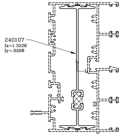
Zero Mull (0400, 1100, 2400 Series)
