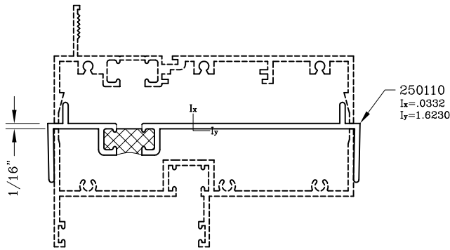
Stack Mull (1500, 2500 Series)
