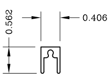
Frame Filler 990427
