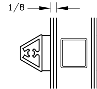
Triple With Trap 1" IG Unit
