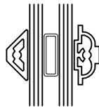
Triple With Trap Exterior Profile Interior 5/8" IG Unit
