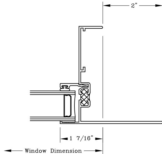
Non Operating Vent Flange Frame #200013
