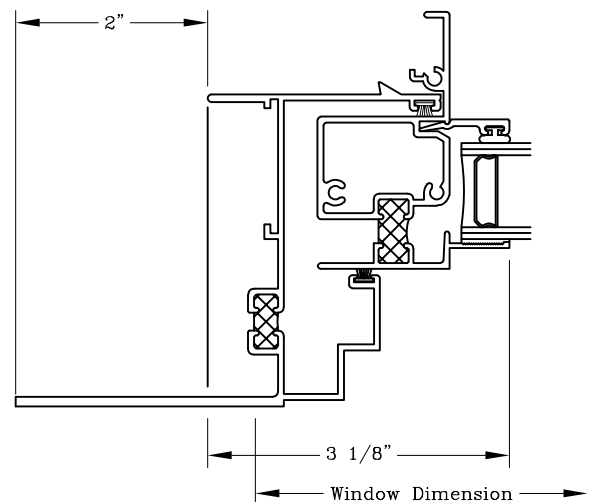
Operating Vent Flange Frame #030033
