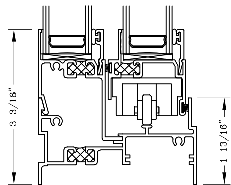
Low Sill Equal Leg #030025
