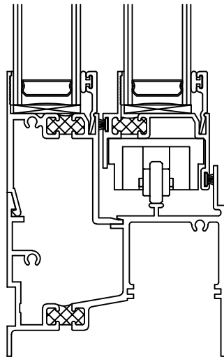
AW Sill Equal Leg #030121
