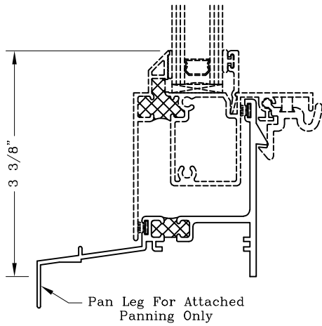
200321 Pan Leg Sill With Spring Latch Barb
