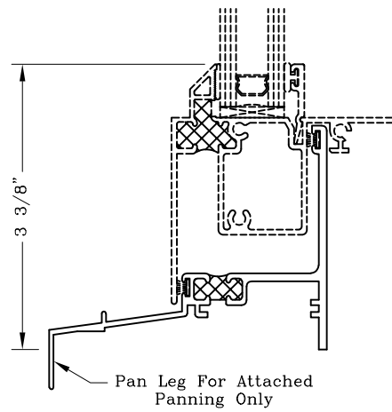
200323 Pan Leg Sill Without Spring Latch Barb
