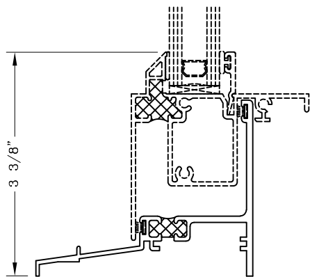
200322 Sill Without Spring Latch Barb
