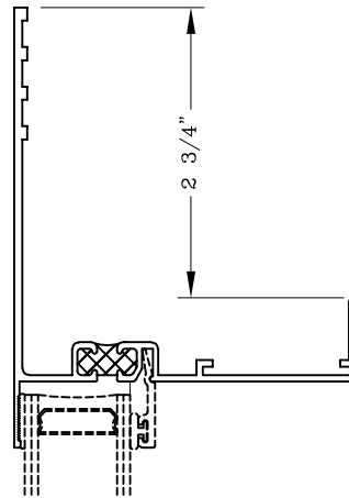
200012 Frame Head w/ 2 3/4” Flange
