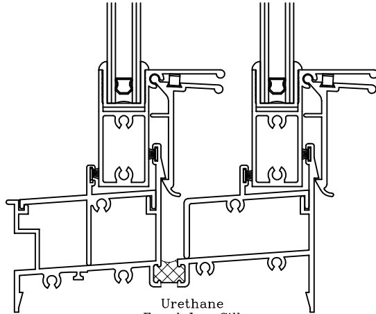
Urethane Equal Leg Sill #240018
