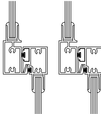
Meeting Rail Single Glaze / Single Glaze
