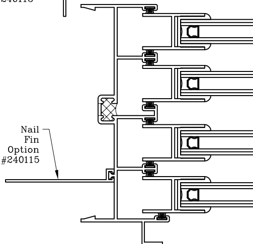
Urethane Sill w/ Nail Fin Option #240018 Nail Fin Option #240115
