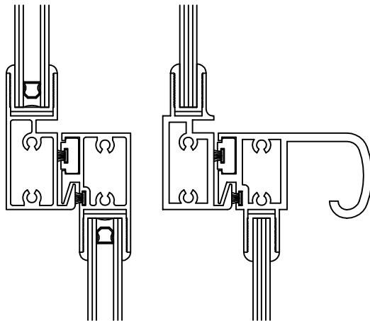
Meeting Rail IG / Single Glaze HC Interior Lock Rail
