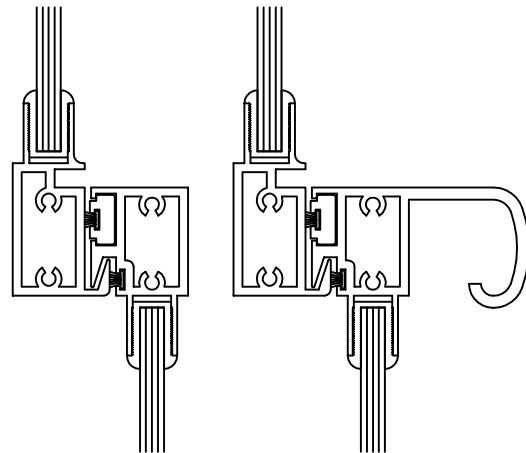
Meeting Rail Single Glaze / Single Glaze HC Interior Lock Rail
