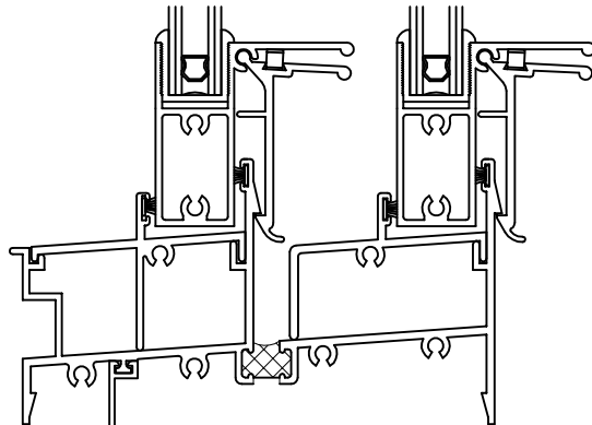
Urethane Sill w/ Nail Fin Option #240018 Nail Fin Option #240115
