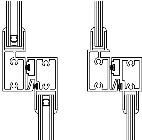
Meeting Rail IG / Single Glaze
