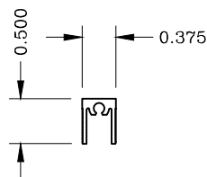
Frame Filler 990290 (For Series 3400)
