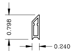
Frame Filler 990397 (Use Only With 990315 Or 990871 Grid)
