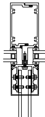
SUNSHADE AT MULLION
