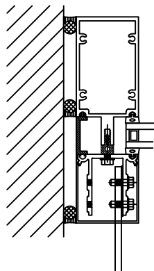
SUNSHADE AT JAMB
