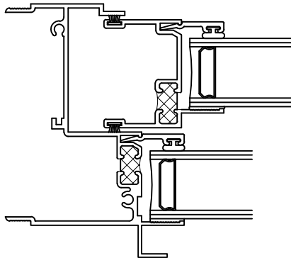
Flat Self-Mull Jamb #203031
