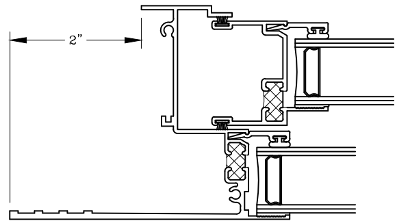
Flat 2" Flange Frame Jamb #200035
