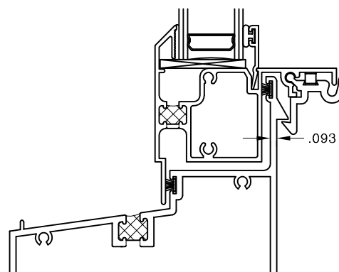
Double Hung Equal Leg Sill w/Spring Latch Barb #221024
