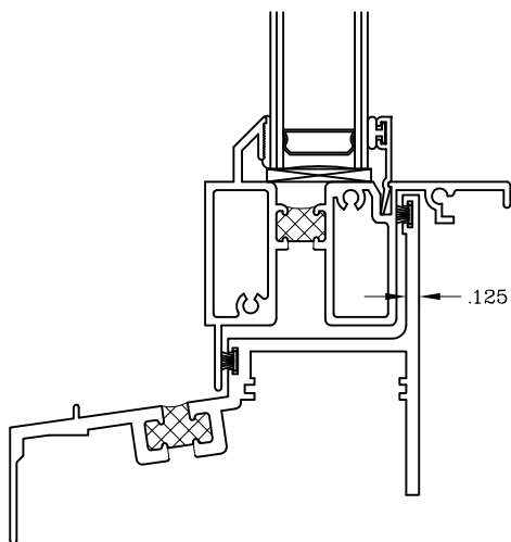
Historic Single Hung Pan Leg Sill #224024
