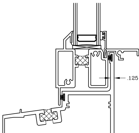
Historic Single Hung Equal Leg Sill #224029
