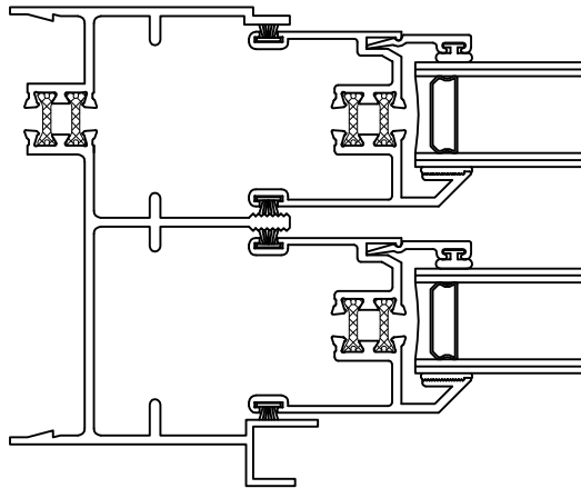
Class "5" Balances Jamb w/ Screen Track #220535
