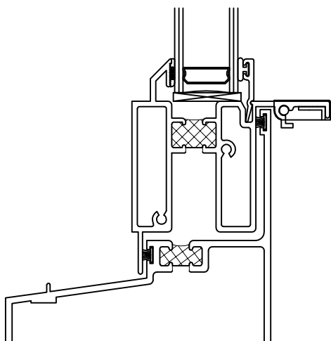
Historic Single Hung Equal Leg 12 PSF Sill #224123
