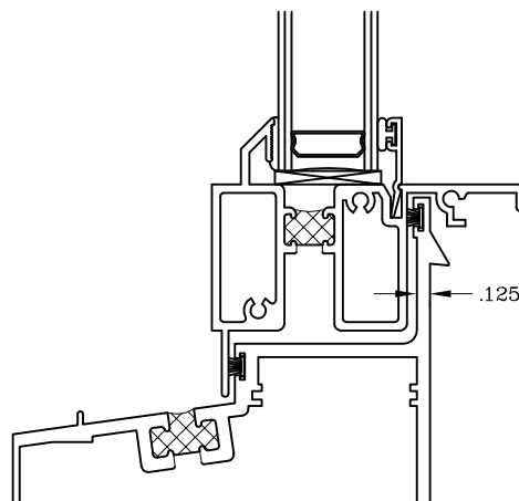
Historic Single Hung Equal Leg Sill w/Spring Latch Barb #224028
