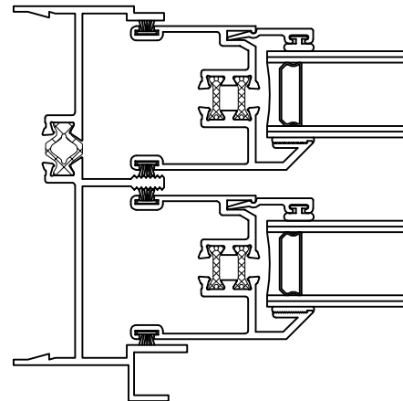
Block and Tackle Jamb w/ Screen Track #220534
