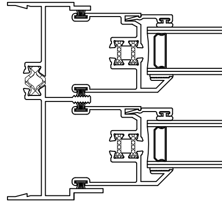
Block and Tackle Jamb w/o Screen Track #220539
