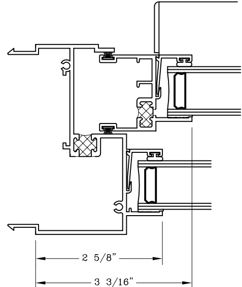
Single Hung Self-Mull Jamb For Block & Tackle Balance Shown With Bead-Glazed Insulated Glass #221037
