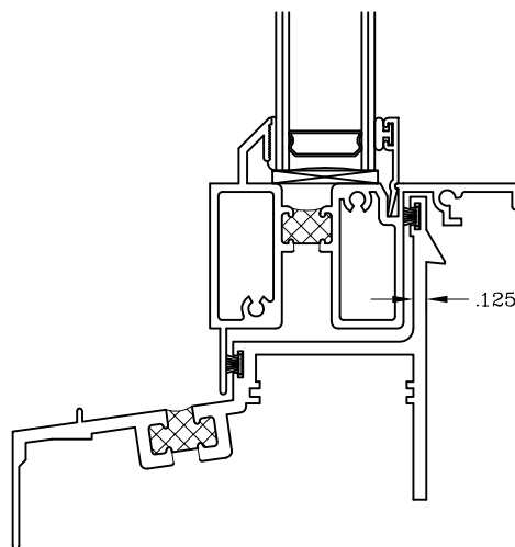
Historic Single Hung Pan Leg Sill w/Spring Latch Barb #224025
