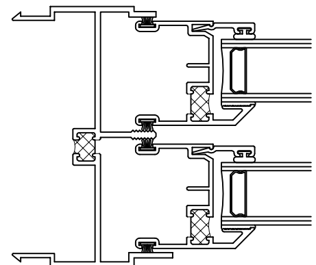
Self-Mull Block & Tackle Jamb w/o Screen Track #221035
