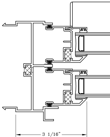
Double Hung Self-Mull Jamb For Block & Tackle Balance Shown With Historic Style Bead-Glazed Glass #221033
