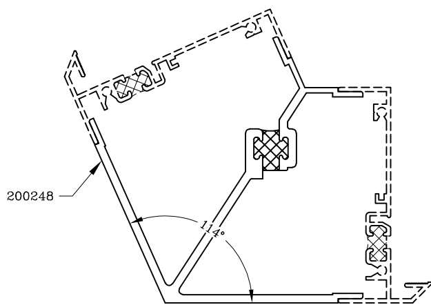
114° Corner Mullion
