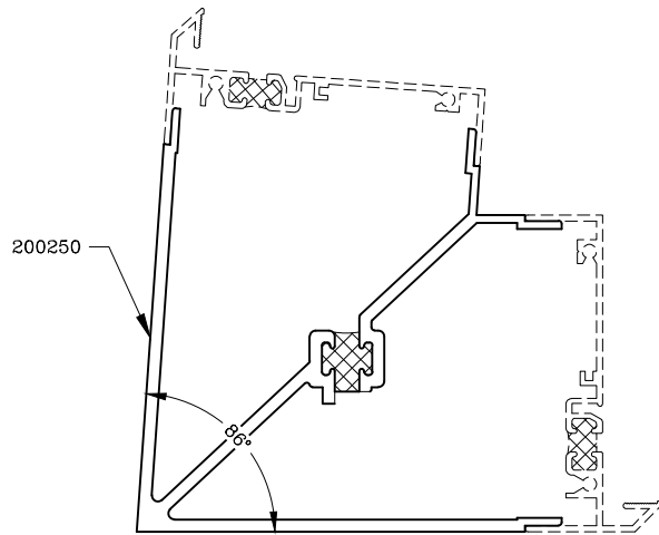
86° Corner Mullion
