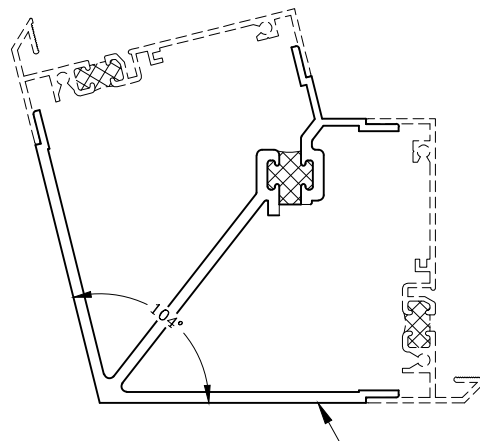
104° Corner Mullion
