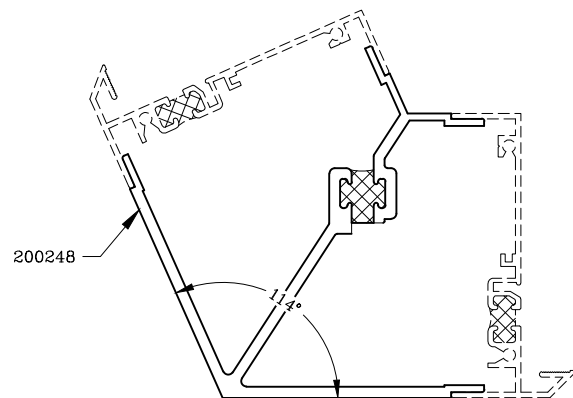
114° Corner Mullion
