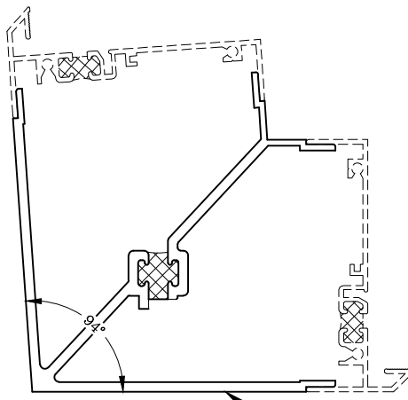
94° Corner Mullion
