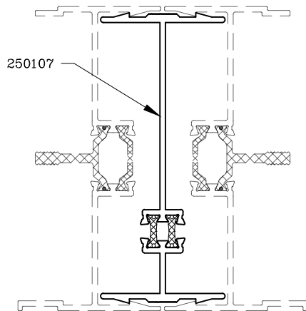
Zero Mullion
