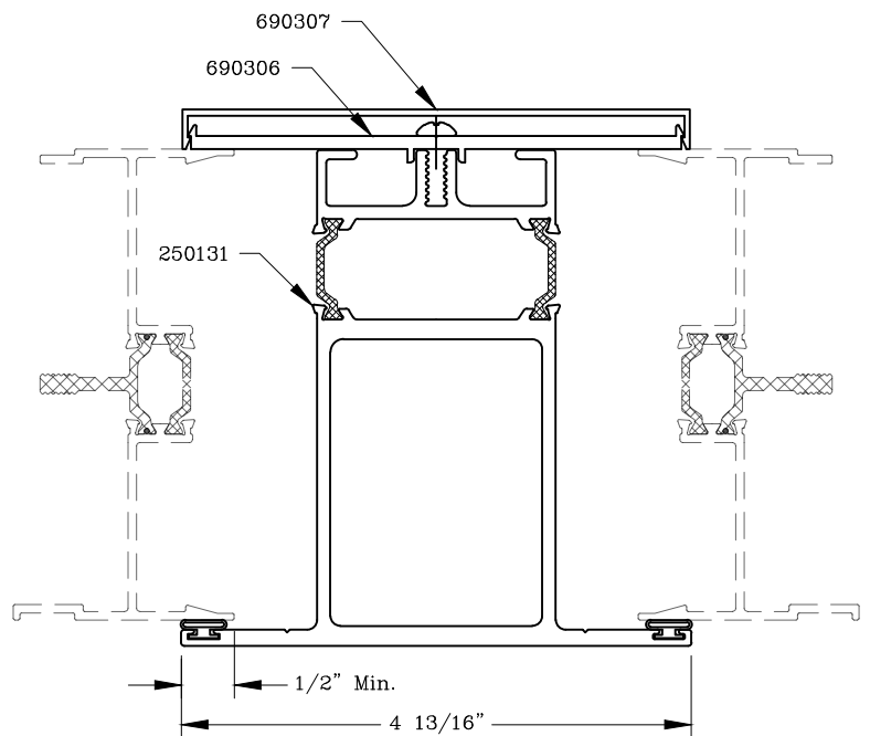
3 Piece Mullion
