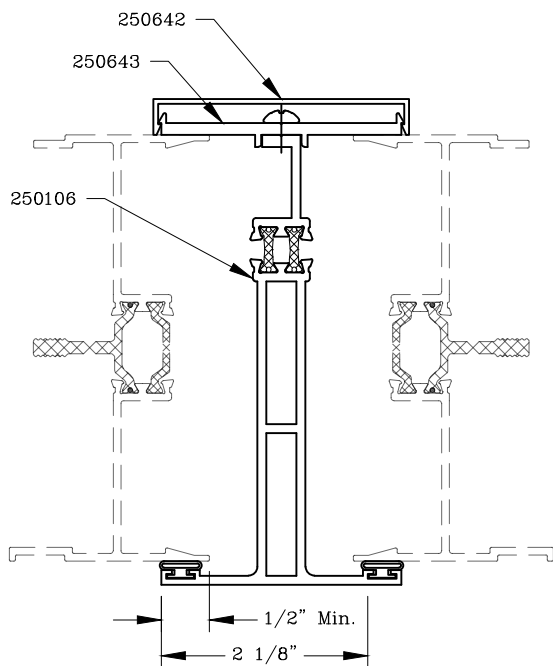
3 Piece Mullion
