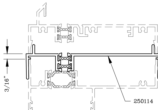
Stack Mullion
