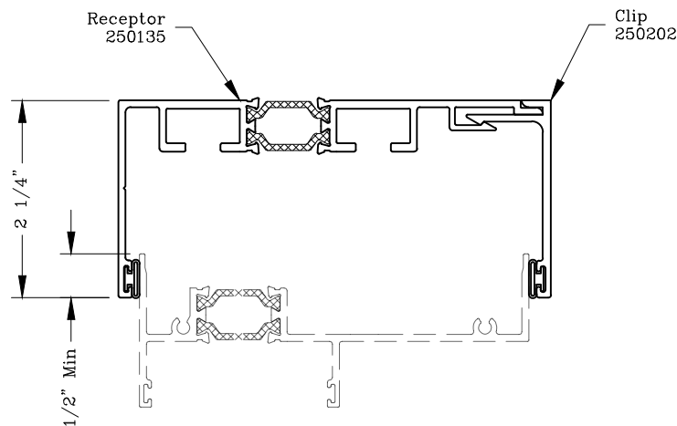
Head/Jamb Receptor
