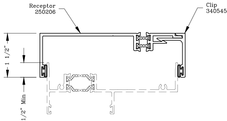
Head/Jamb Receptor
