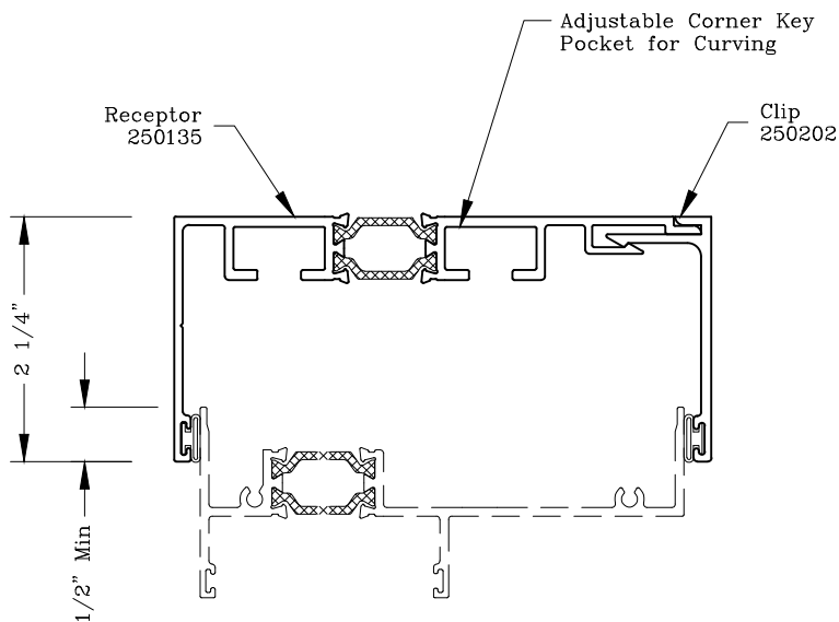
Head/Jamb Receptor
