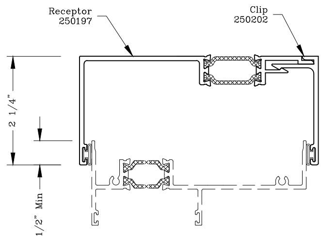
Head/Jamb Receptor
