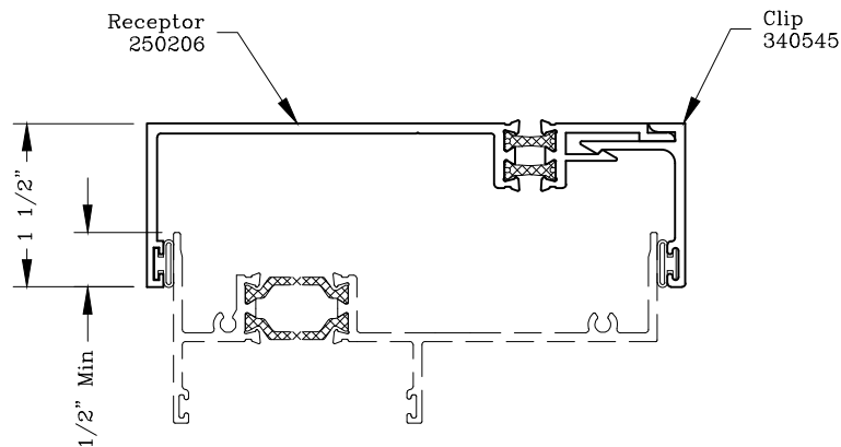
Head/Jamb Receptor
