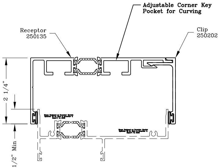
Head/Jamb Receptor
