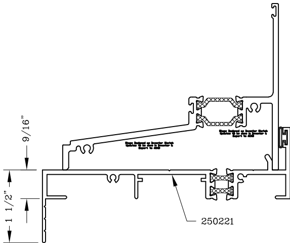
Sill Starter
