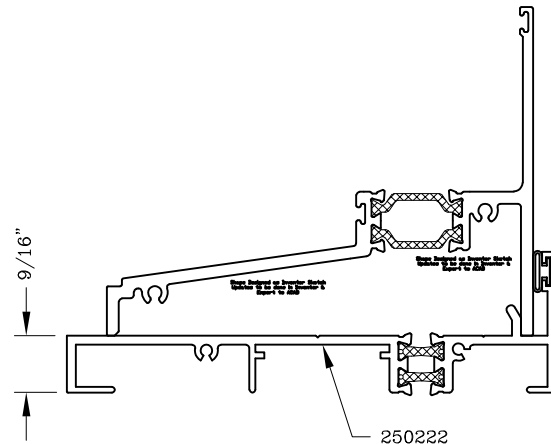
Sill Starter
