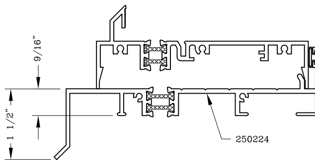
Sill Starter
