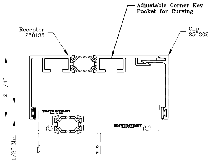
Head/Jamb Receptor
