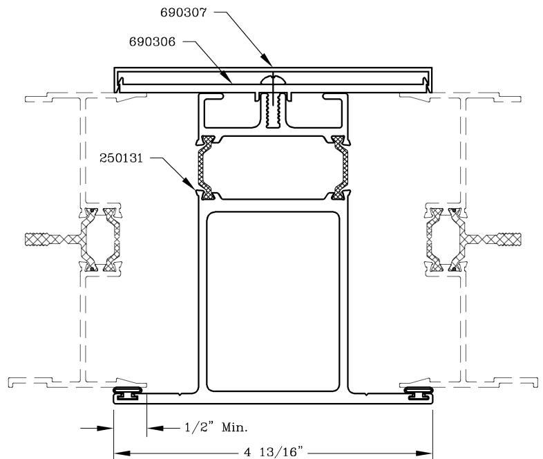
3 Piece Mullion
