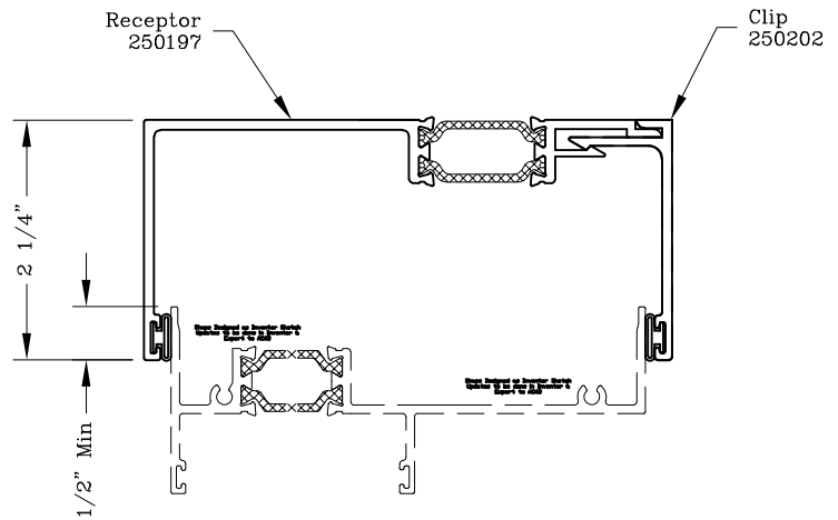
Head/Jamb Receptor
