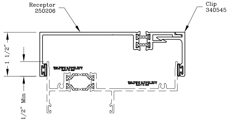
Head/Jamb Receptor
