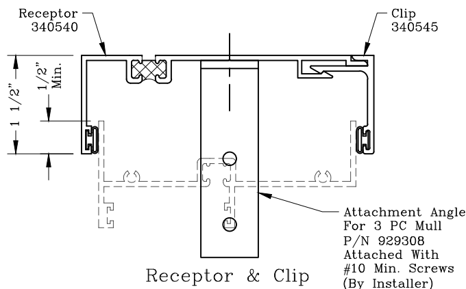
Tube Stack Mull
