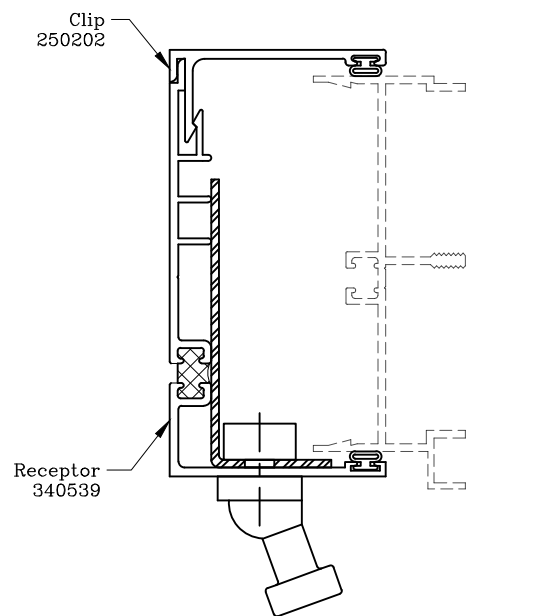
Receptor & Clip (To Be Used In Applications Requiring Window Cleaner Bolts)
