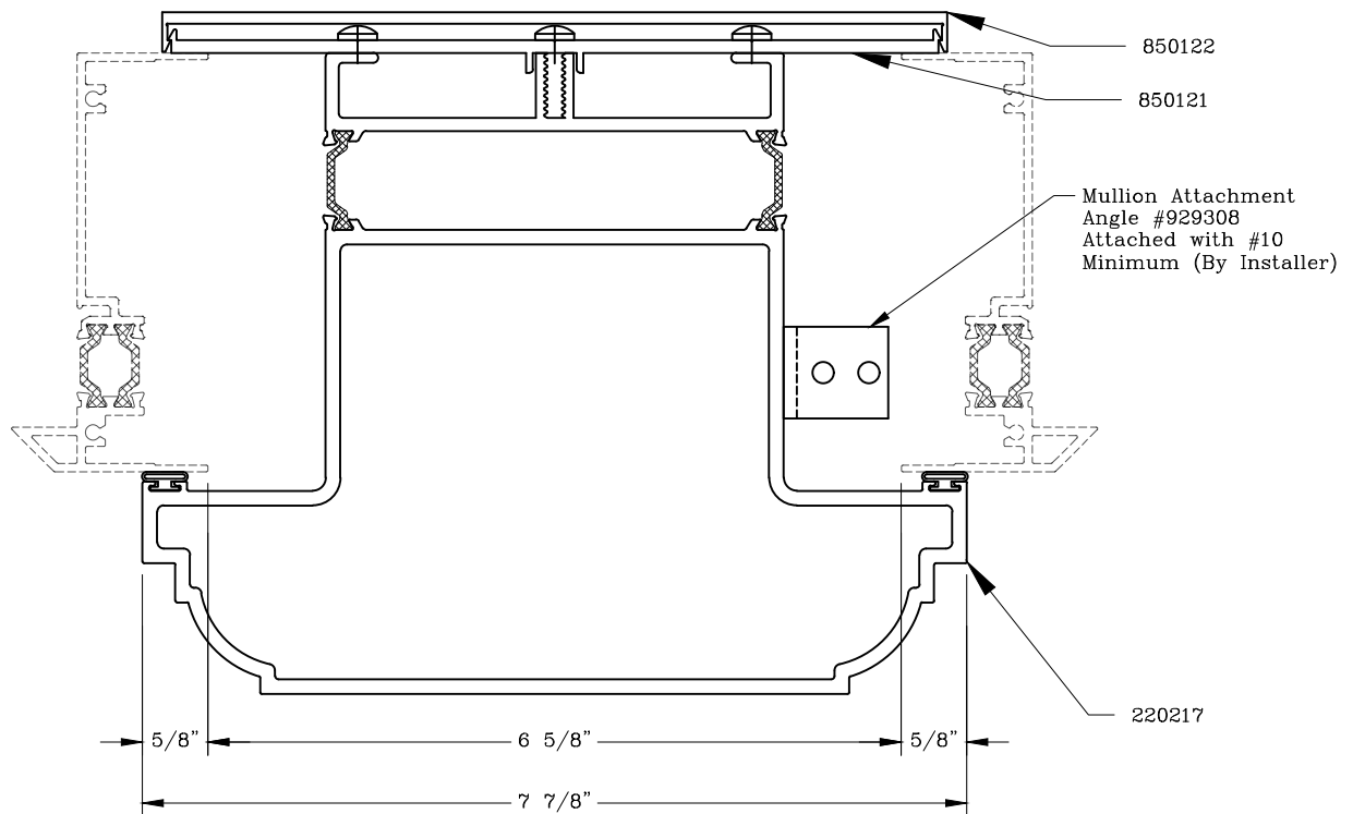
3 Piece Mullion – Profile
