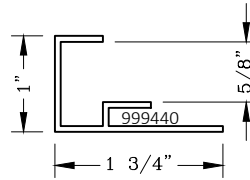
5/8" Drywall Trim
