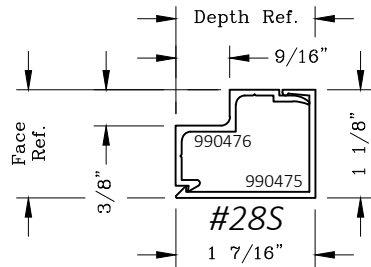
5/8" Drywall Trim
