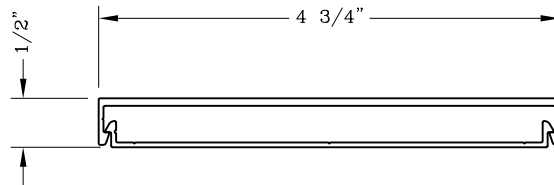
853142 4 3/4" Mullion Cover
