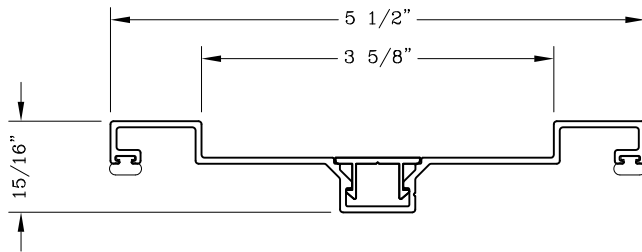
850348 Mullion Cap
