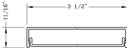
851639 3 1/2" Mullion Cover
