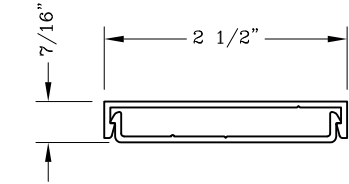
850362 2 1/2" Mullion Cover
