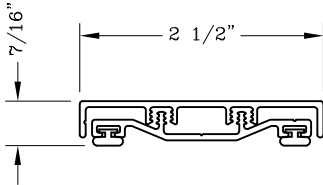
859043 2 1/2" Mullion Cover Press Fit
