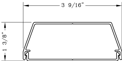
857866 3 1/2" Beveled Mullion Cover
