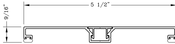
850348 Mullion Cap
