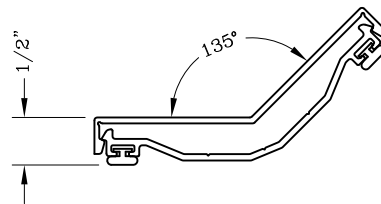
855664 45° Mullion Cover
