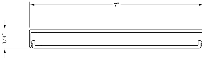
852831 7" Mullion Cover
