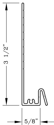
856515 HEAD / JAMB SHALLOW PANNING
