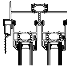
Detail Scale 1:4
