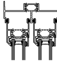
Detail Scale 1:4
