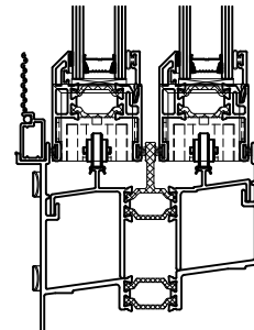
Detail Scale 1:4
