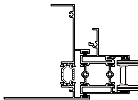
Shown With Pull Rail Stile Detail Scale 1:4
