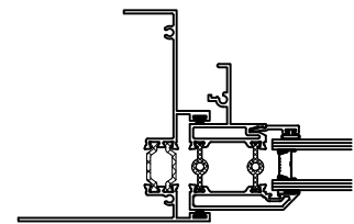
Shown With Pull Rail Stile Detail Scale 1:4
