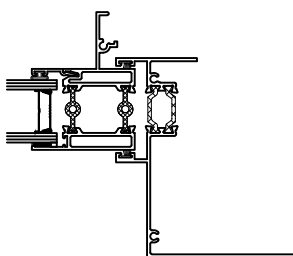
Shown With Pull Rail Stile Detail Scale 1:4
