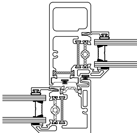
1" IG Historic AW 40 Rated OX – Shown XO – Opposite
