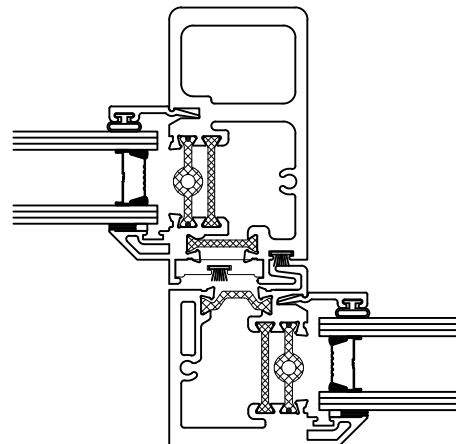
1" IG Historic AW 40 Rated OXO Left Slide – Shown OXO Right Slide – Opposite
