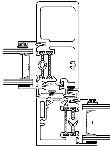
1 1/4" IG Non Historic AW 50 Rated OXO Left Slide – Shown OXO Right Slide – Opposite
