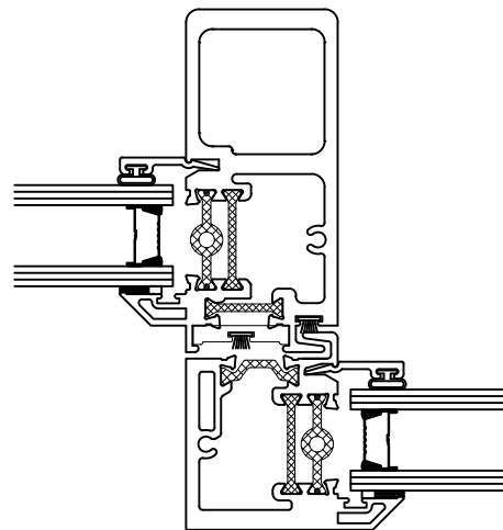
1" IG Historic AW 50 Rated OXO Left Slide – Shown OXO Right Slide – Opposite
