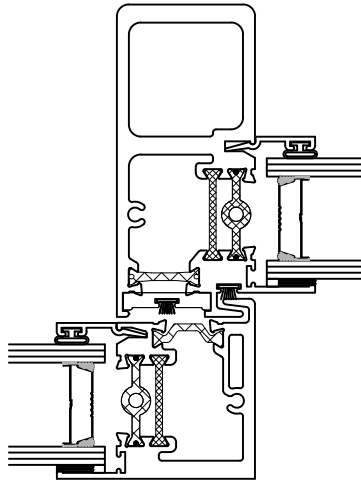
1 1/4" IG Non Historic AW 50 Rated OX – Shown XO – Opposite
