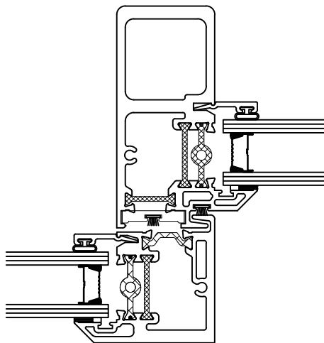
1" IG Historic AW 50 Rated OX – Shown XO – Opposite
