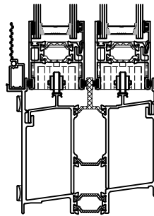
Detail Scale 1:4
