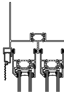
Detail Scale 1:4
