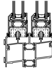
Detail Scale 1:4
