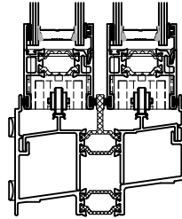
Detail Scale 1:4
