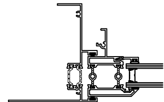
Shown With Pull Rail Stile Detail Scale 1:4
