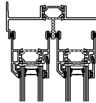
Detail Scale 1:4
