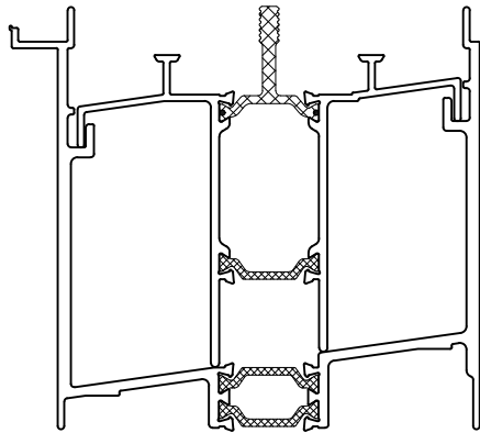
15 PSF Equal Leg Sill With Screen Track
