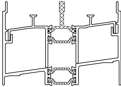
10 PSF Equal Leg Sill
