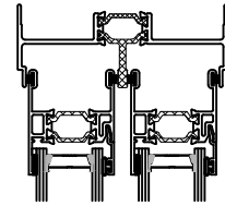
Detail Scale 1:4
