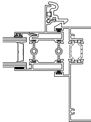
1 1/4" IG Non Historic Vent Stile With Extruded Spring Latch
