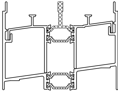
12 PSF Equal Leg Sill
