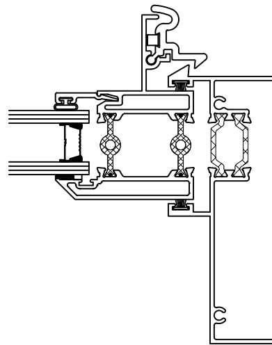
1" IG Historic Vent Stile With Extruded Spring Latch
