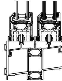
Detail Scale 1:4
