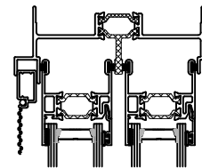
Detail Scale 1:4
