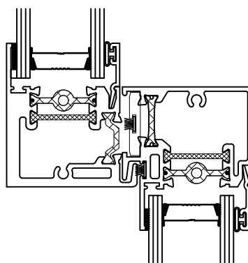
1 1/4" Flat Glazing A.W. 50
