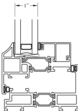
GT6700FFC Concave
