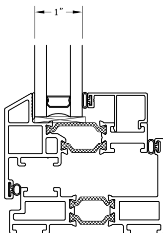
GT6700FFB Beveled
