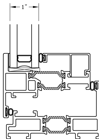
GT6700FFF Flat
