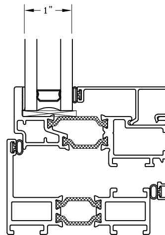
GT6700F Flat
