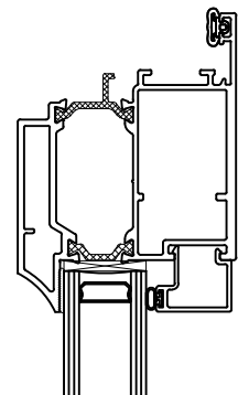
Concave Profile
