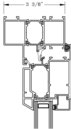
3 3/8" Frame
