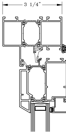
3 1/4" Frame
