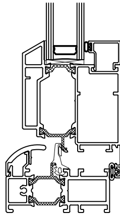
Beveled Profile
