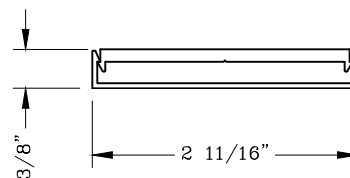
990900 Mullion Clip
