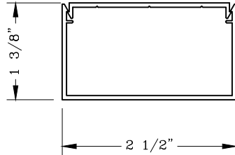
990911 Mullion Clip
