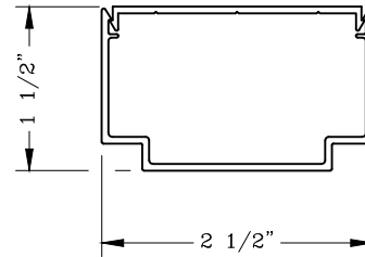
990911 Mullion Clip
