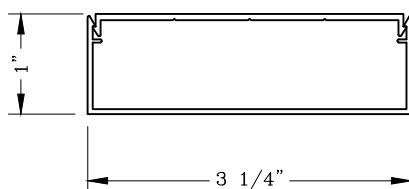
990907 Mullion Clip
