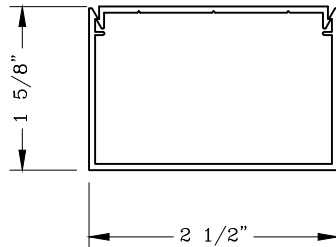
990911 Mullion Clip
