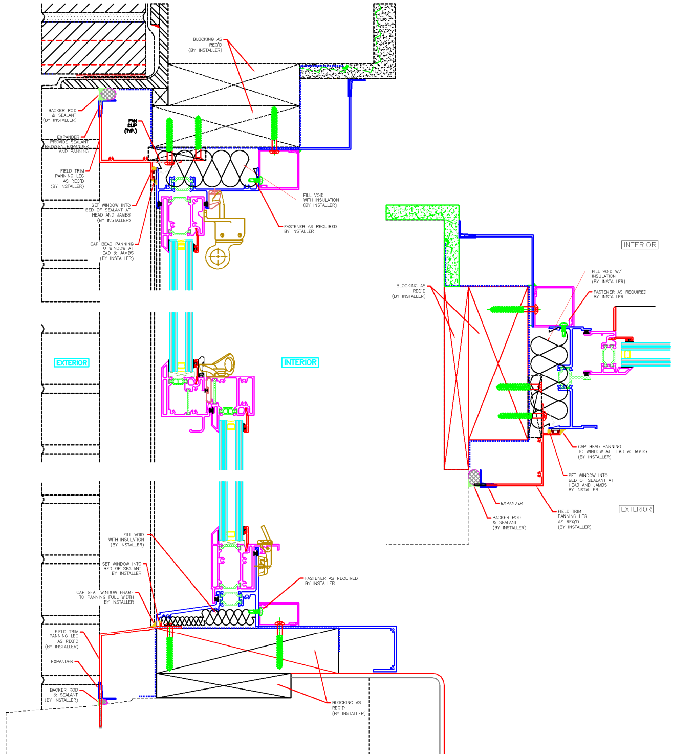
Figure #11 – Installation Drawing Example
