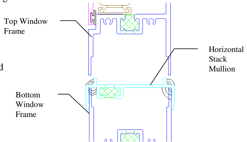
Figure # 24 Top Window frame set in place
