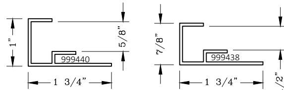
5/8" Drywall Trim 1/2" Drywall Trim
