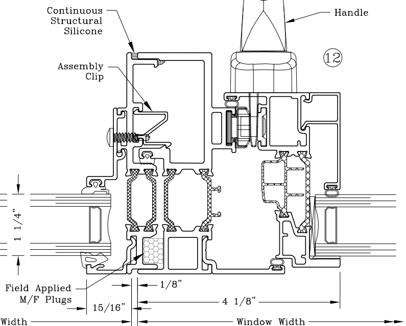
Male/Female Fixed Exterior Glazed/Project-In (Casement Shown)
