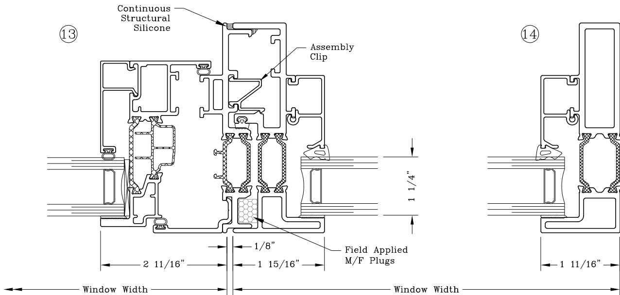
Male/Female Project-In/Fixed Interior Glazed (Casement Shown)
