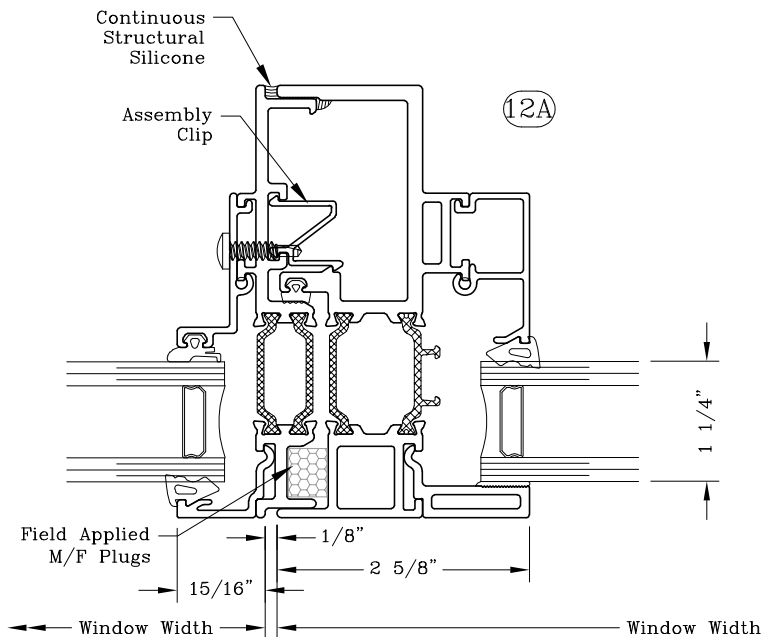
Male/Female Fixed Exterior Glazed/Project-In Fixed
